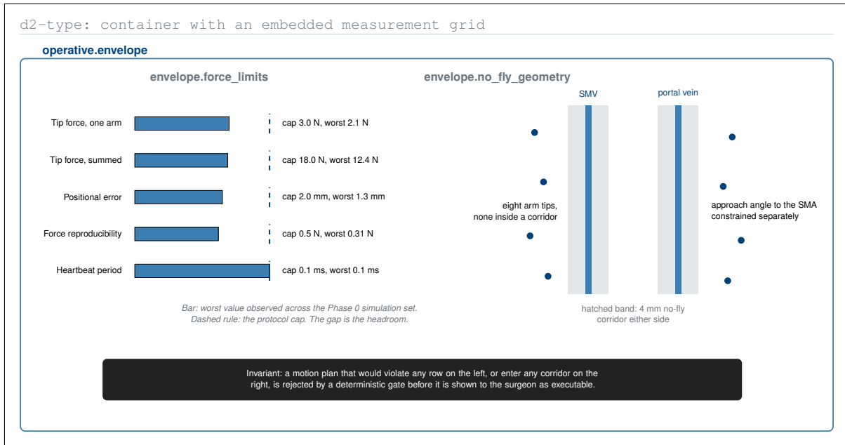
Figure 20. The operative envelope drawn as two sibling containers, the force limits with their observed headroom on the left and the vascular no-fly geometry on the right, joined by the deterministic gate that rejects any plan violating either of them.
